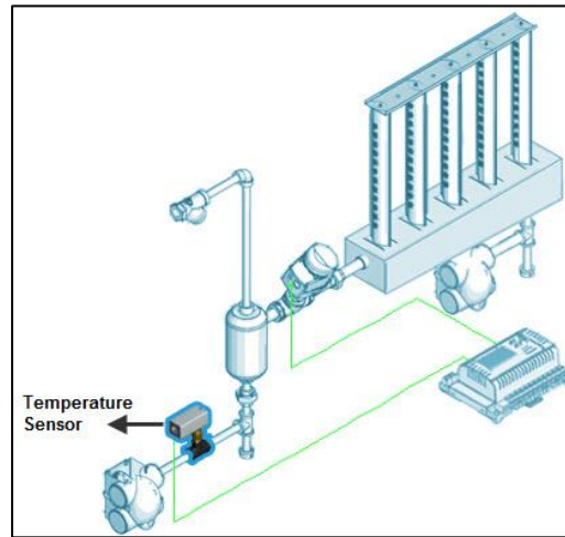
Illustration 14 - Temperature Sensor Installation
