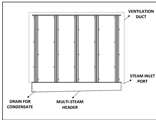
Illustration 6 - Manifold Installation: Side View
