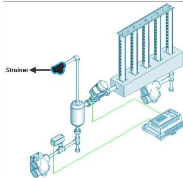
Illustration 17 - Strainer Installation
