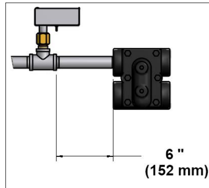
Illustration 16 - Correct distance between Temperature Sensor and Steam Trap
