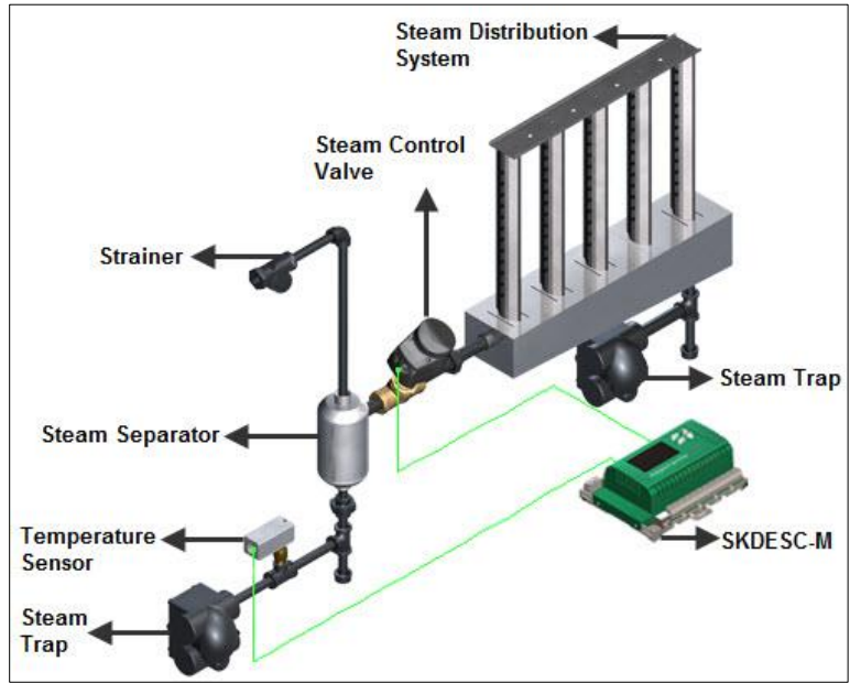
Illustration 2 - Components Overview
