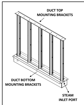
Illustration 7 - Header Mounting Brackets and Steam
