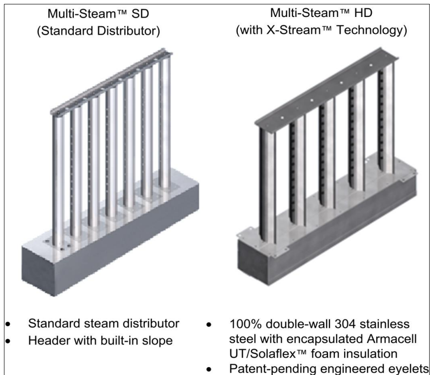
Illustration 1 - X-Stream and Standard Steam Distributor
