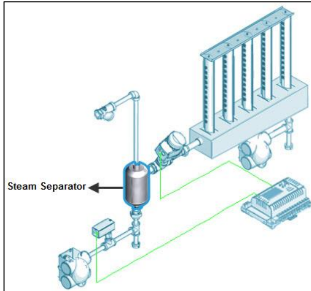
Illustration 11 - Steam Separator Installation
