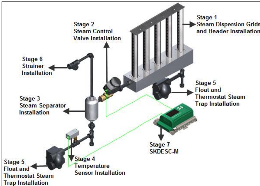
Illustration 3 - Installation Stages Overview
