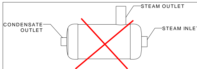
Illustration 13 - Incorrect Installation
