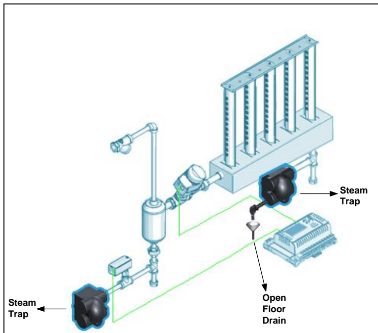
Illustration 15 - Float and Thermostatic Steam Trap Installation
