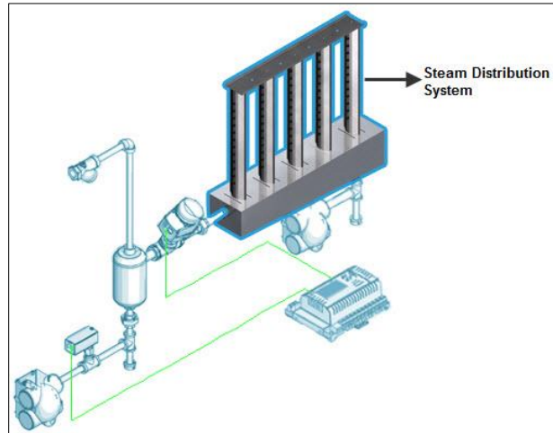
Illustration 4 - Steam Distribution System Installation
