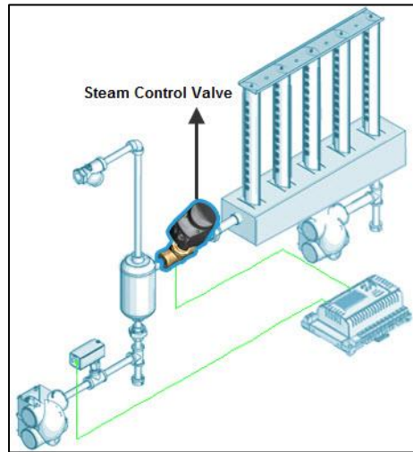
Illustration 8 - Steam Control Valve Installation
