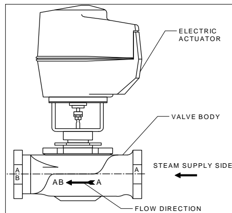
Illustration 9 - Flow Direction, Steam Control Valve
