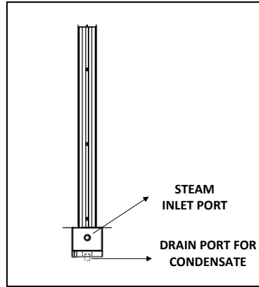
Illustration 5 - Manifold Installation: Front View
