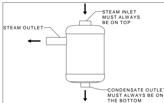
Illustration 12 - Correct Installation
